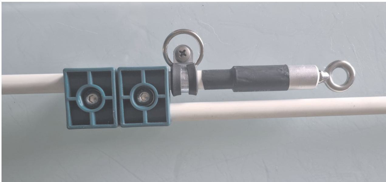
Fastening of the extended arm 40m kit
