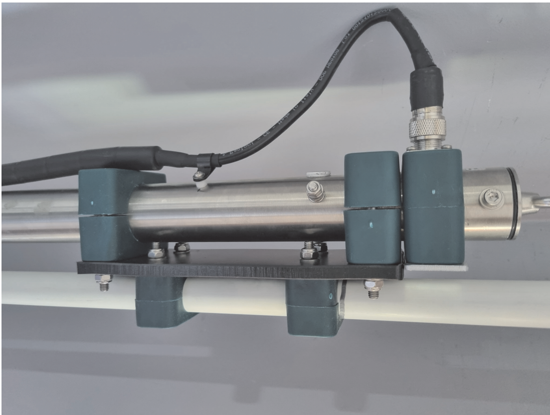
Center post extension arm
